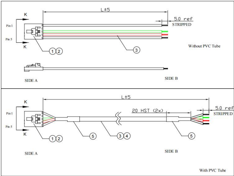
Wire Harness With PVC Tube (Without Shielding)
