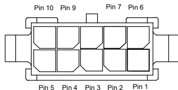
430201000 SHOWN VIEW K-K 2:1
