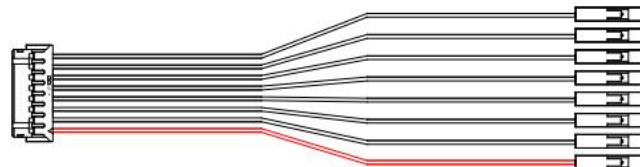
PHD TO DuPont 2.54 Discrete Single Pin (散PIN) TYPE PHD-DX
