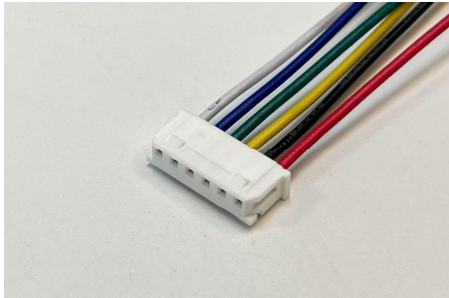
Wire Harness Assembly
